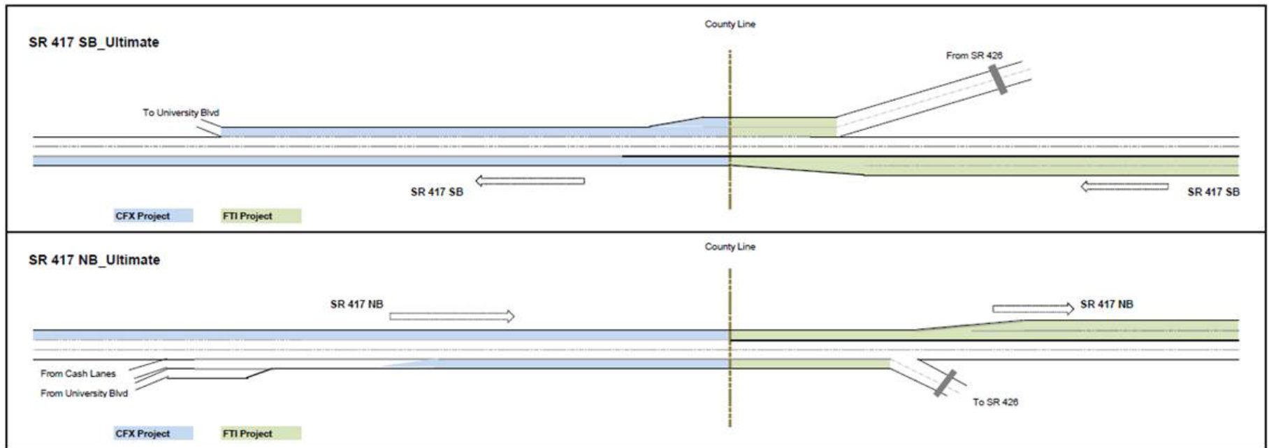
Figure 9: SR 417/Seminole Expressway Ultimate Lane Configuration
