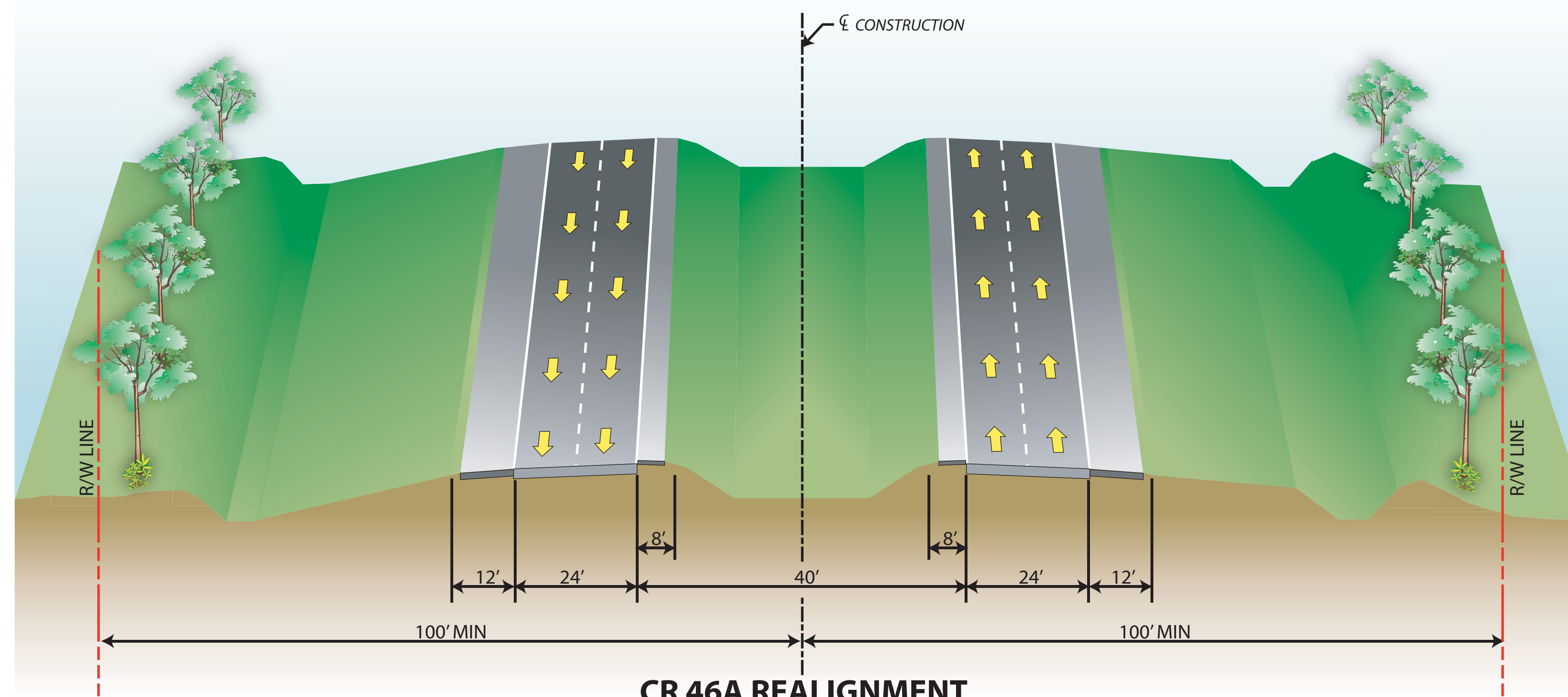
CR 46A REALIGNMENT 4-LANE RURAL SECTION
