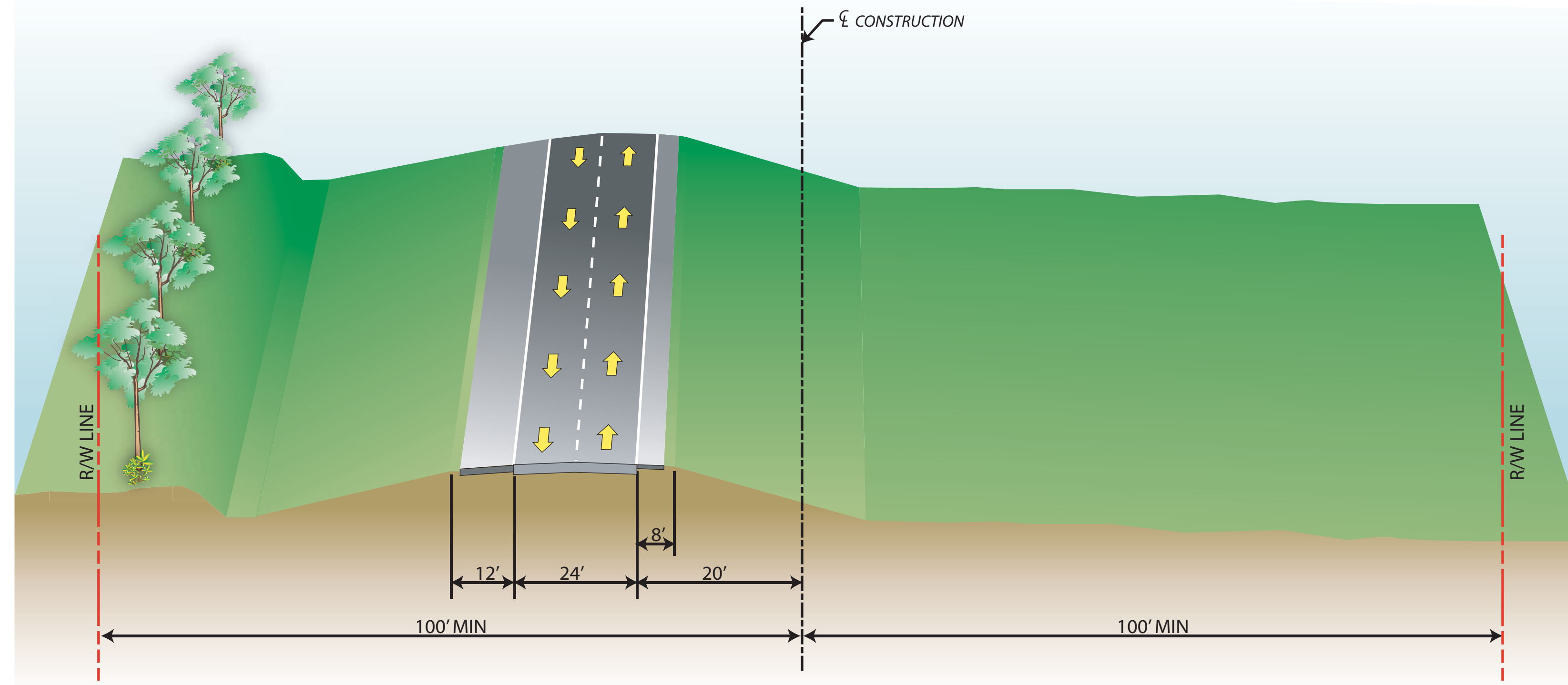
CR 46A REALIGNMENT 2-LANE RURAL SECTION
