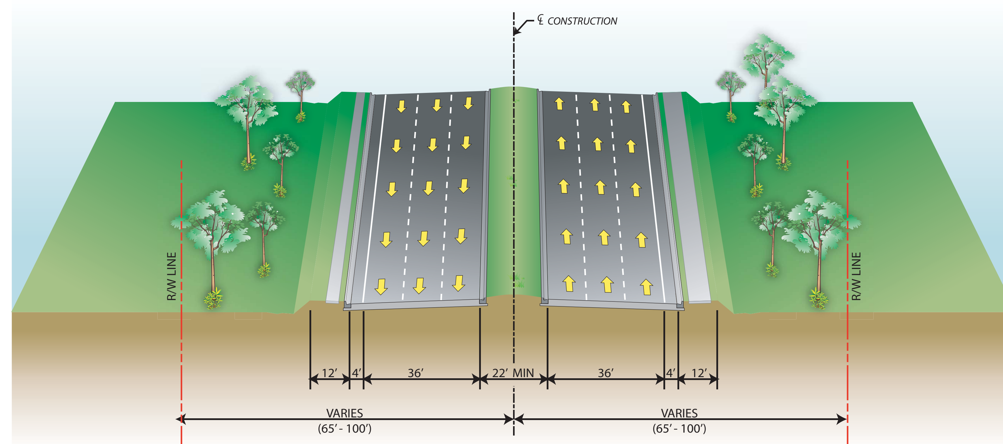
SR 46 CORRIDOR IMPROVEMENTS 6-LANE DIVIDED URBAN SECTION
