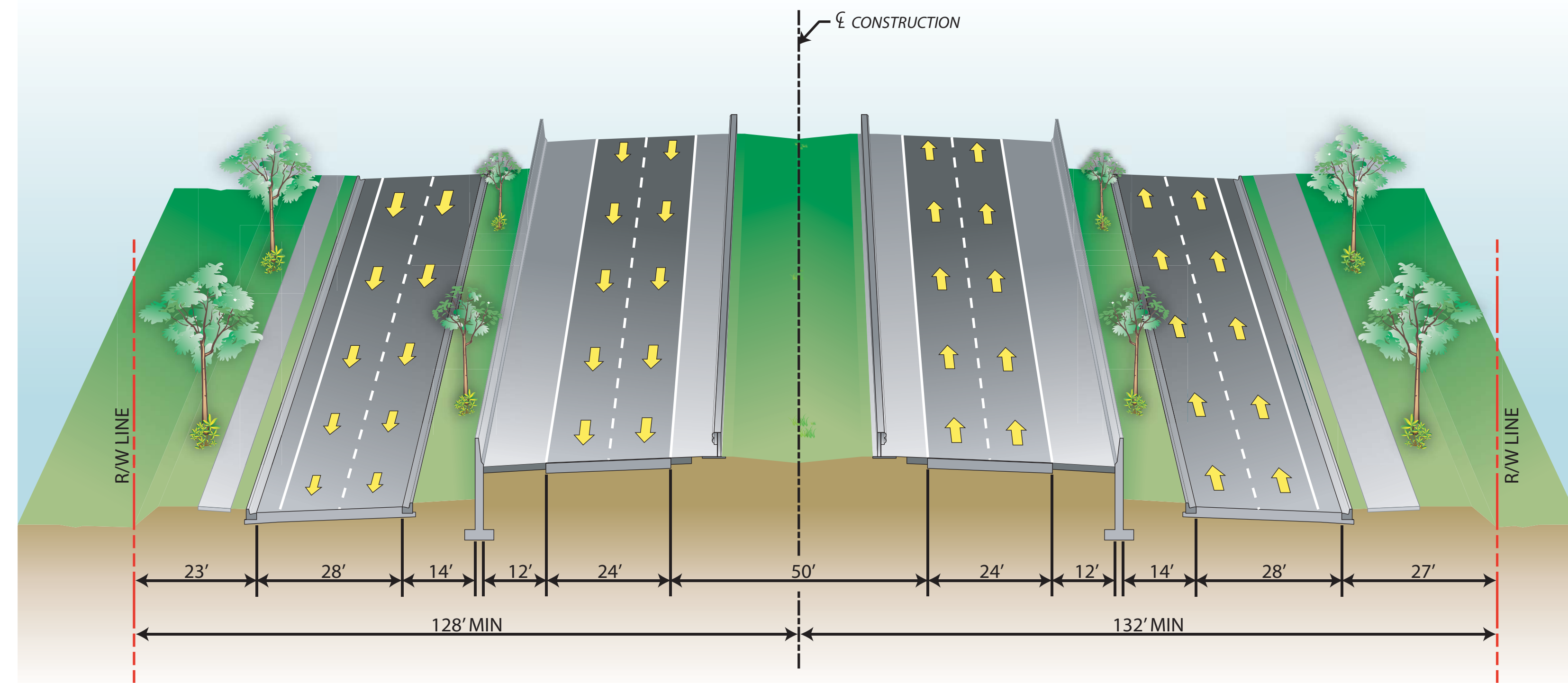
WEKIVA PARKWAY 4-LANE EXPRESSWAY WITH FRONTAGE ROADS
