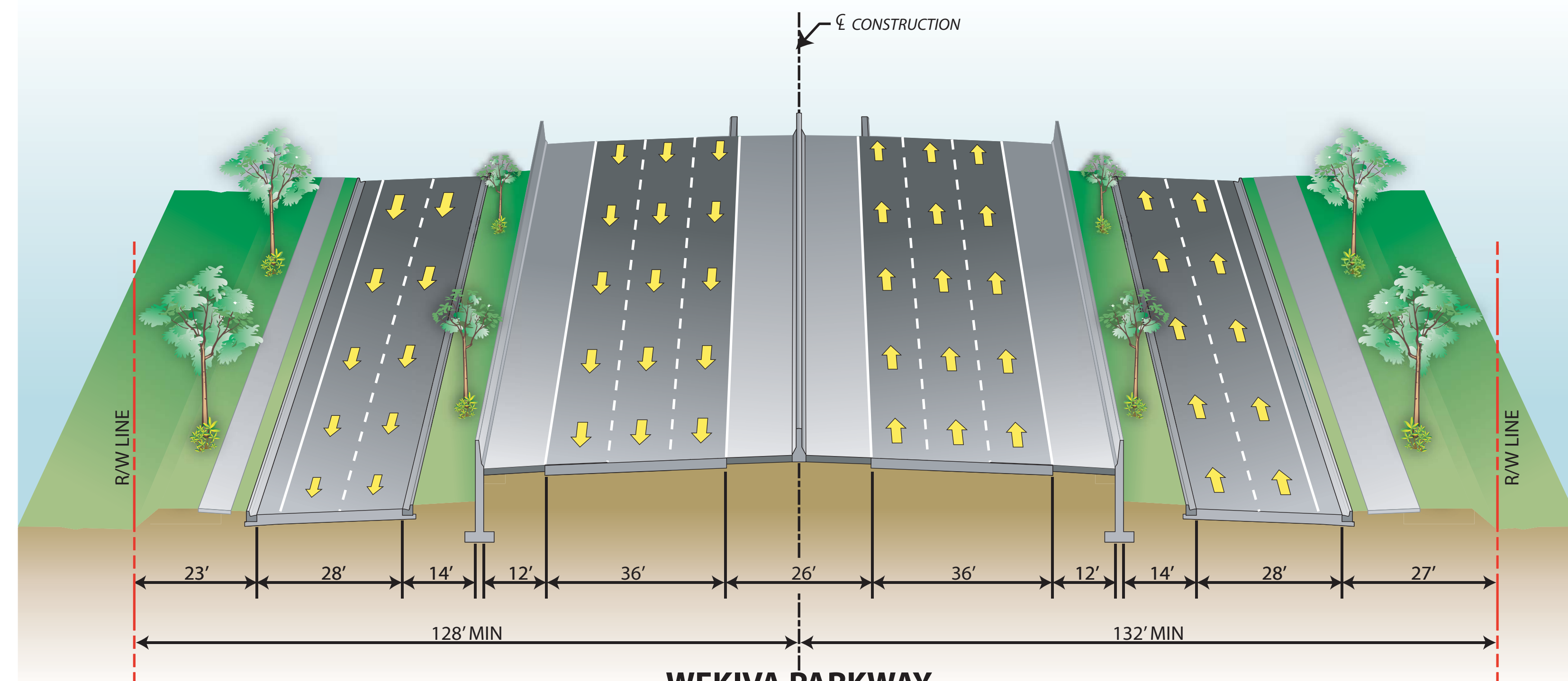
WEKIVA PARKWAY ULTIMATE 6-LANE EXPRESSWAY WITH FRONTAGE ROADS
