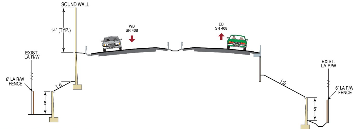
SOUND WALL TYPICAL SECTION
