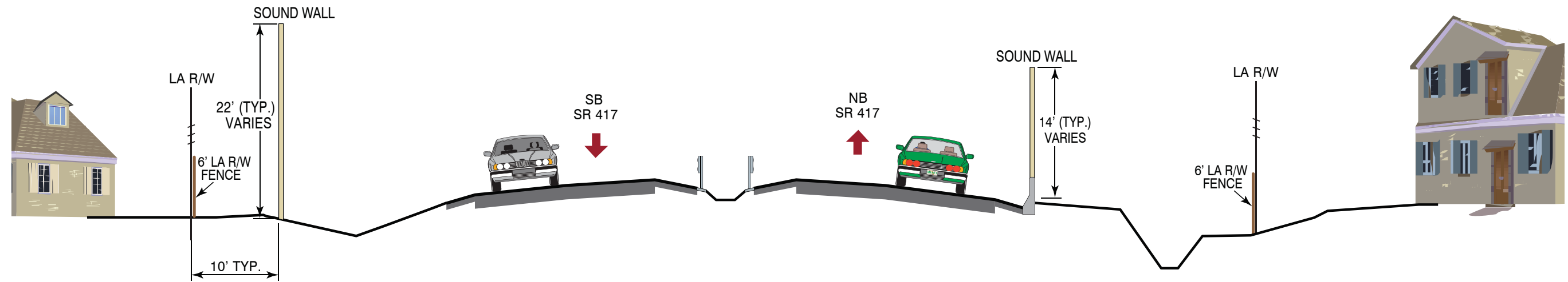
SOUND WALL TYPICAL SECTION
