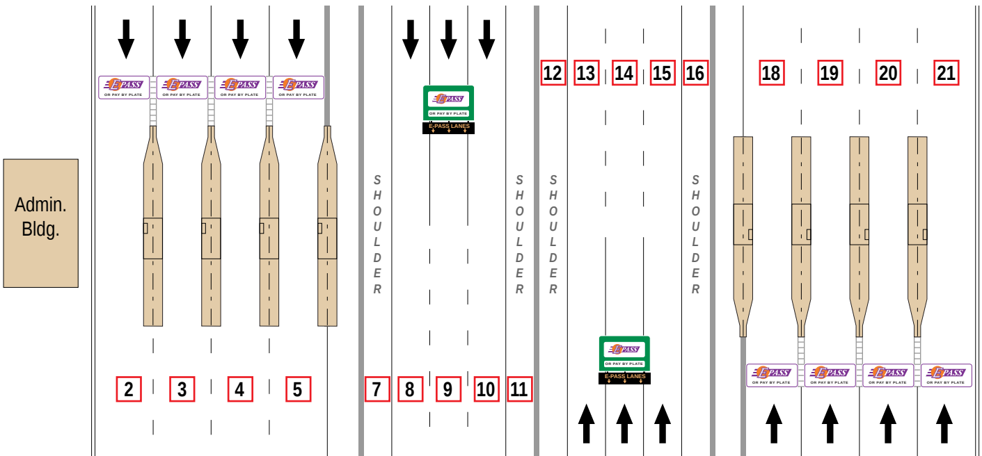
Curry Ford Mainline Toll Plaza Elevation
