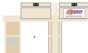
Semoran Boulevard/Yucatan Drive On Ramp Toll Plaza Elevation
