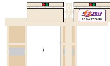
Bumby Avenue On and Off Ramp Toll Plaza Elevation
