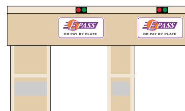
East Colonial Drive On and Off Ramp Toll Plaza Elevation
