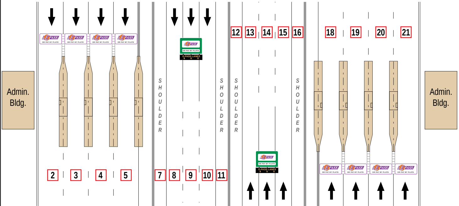
Pine Hills Mainline Toll Plaza Elevation
