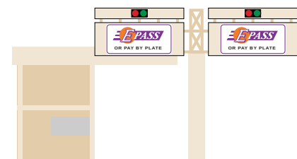
New Independence Parkway On and Off Ramp Toll Plaza Elevation
