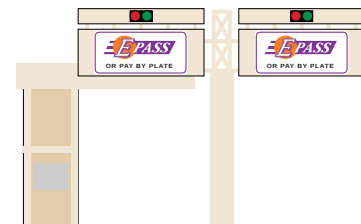
Conway Road On Ramp Toll Plaza Elevation
