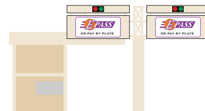
Old Winter Garden Road On and Off Ramp Toll Plaza Elevation
