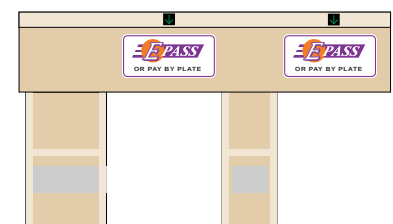
Plant Street / Franklin Street On Ramp Toll Plaza Elevation
