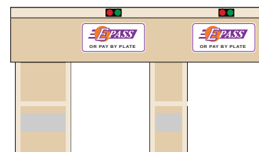
Leevista Boulevard On and Off Ramp Toll Plaza Elevation
